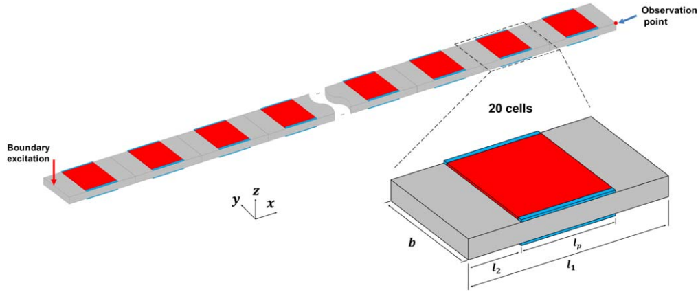
Figure 5. A spatial periodic waveguides containing 20 active units.
