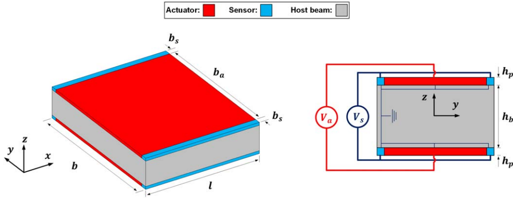
Figure 1. The designed active unit.
