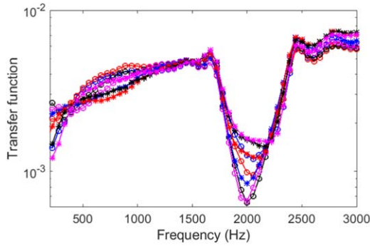
Figure 14. Influences of the initial phase \varphi_0 of the modulation wave on the transfer function. The excitation is applied on the left in each simulation.
