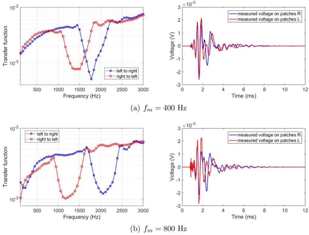
Figure 12. Left panel: left to right and right to left transfer functions of the waveguide. Right panel: measured voltage on patches ‘R’ and ‘L’ due to the excitation on patches ‘L’ and ‘R’. The modulation parameters are \alpha_1 = 0 , \alpha_2 = 2 , and (a) f_m = 400 Hz, (b) f_m = 800 Hz.
